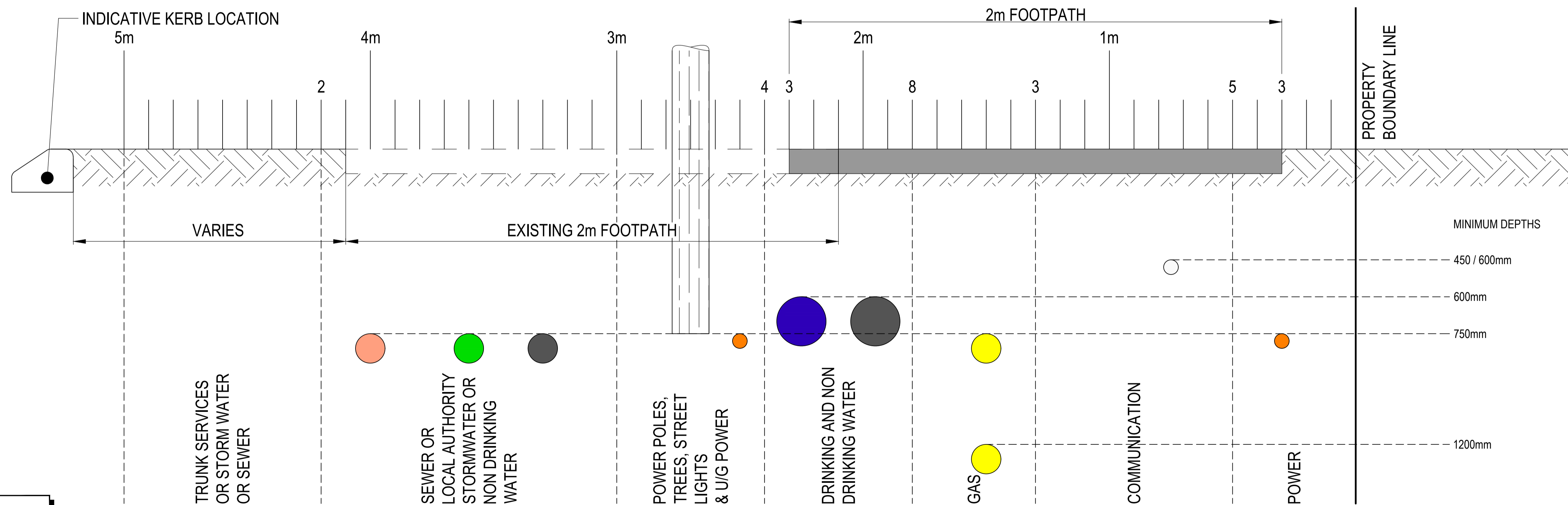
ROAD RESERVE ALLOCATION FOR UTILITY SERVICES AND FOOTPATH ALIGNMENT SCALE 1:10
