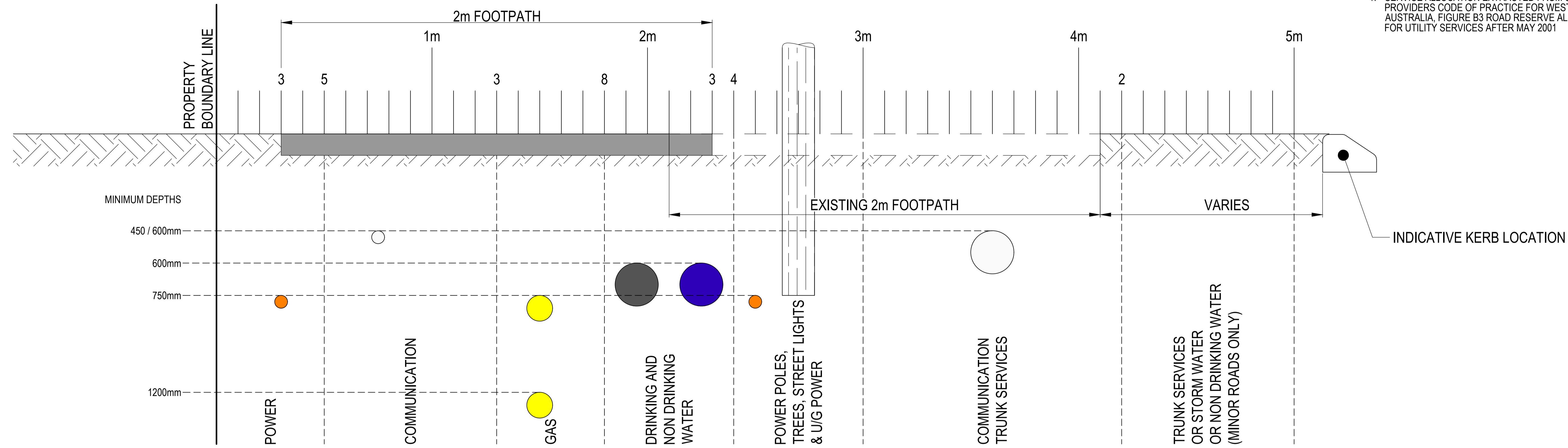
ROAD RESERVE ALLOCATION FOR UTILITY SERVICES AND FOOTPATH ALIGNMENT SCALE 1:10
